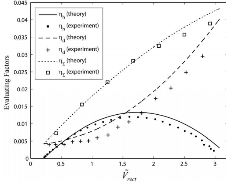
Figure 9. Theoretical and experimental results on three evaluating factors in PHE with SSHI interface.
